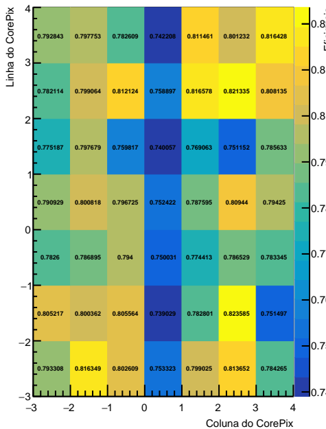
\epsilon_2^1(\text{CP0}): \text{Jan24-Mar6}
