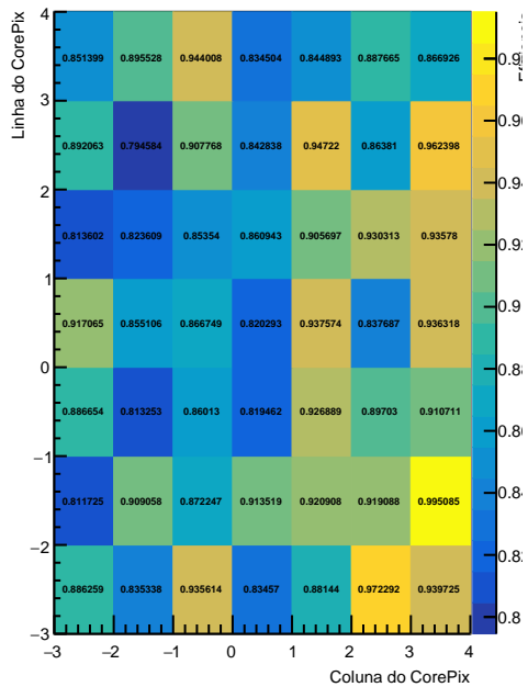
\epsilon_1^1(\text{CP0}): \text{Apr24-May14}
