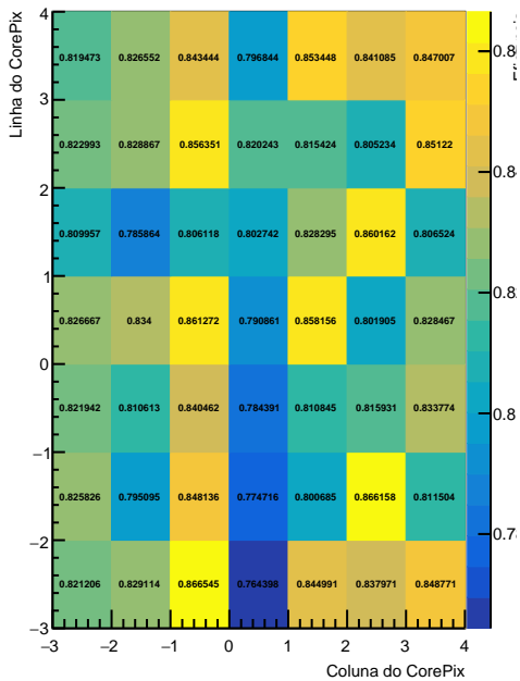
\epsilon_2^1(\text{CP0}): \text{Apr24-May14}
