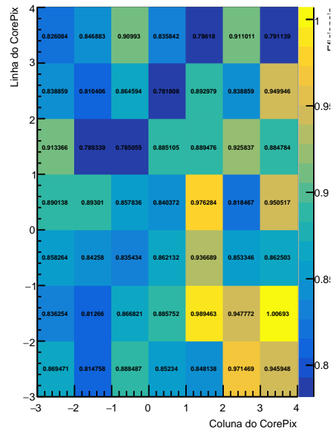
\epsilon_3^1(\text{CP0}): \text{Apr24-May14}
