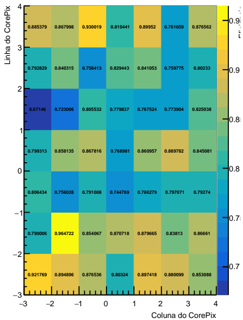
\epsilon_1^2(\text{CP0}): \text{Jun\_12\_Nov\_1\_2022.root}
