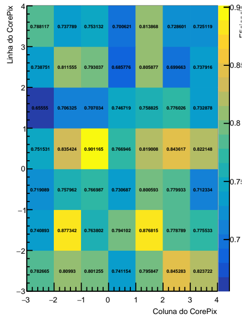
\epsilon_3^2(\text{CP0}): \text{Jun\_12\_Nov\_1\_2022.root}
