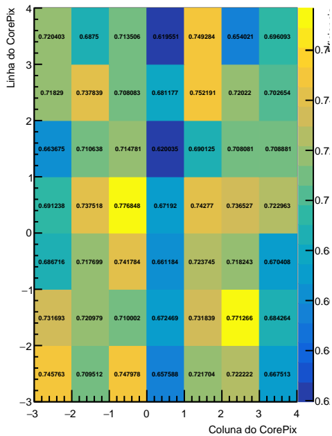
\epsilon_2^2(\text{CP0}): \text{Jun\_12\_Nov\_1\_2022.root}
